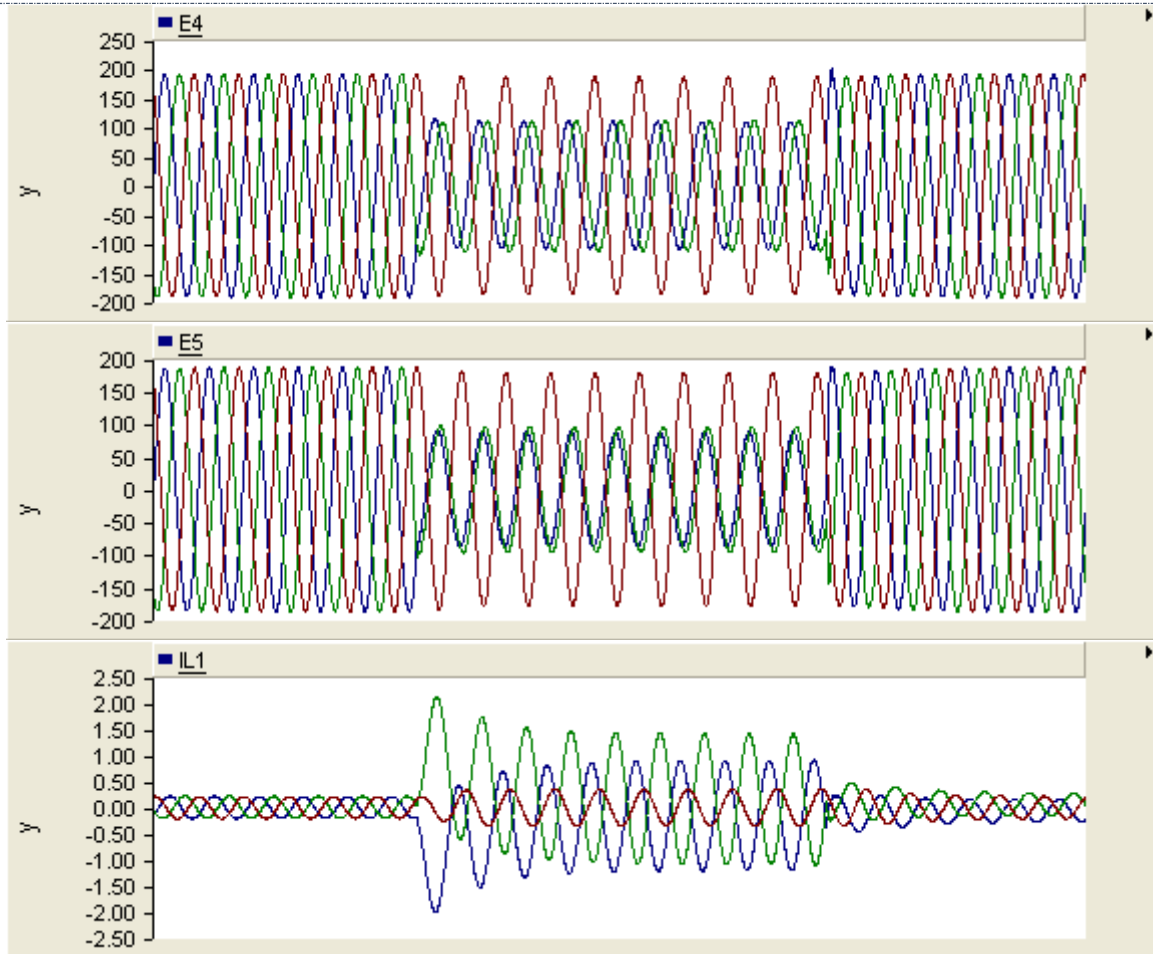
Discrete wavelet transform Decomposition results for various frequency bands AG fault 0 degree 0.5M locations
