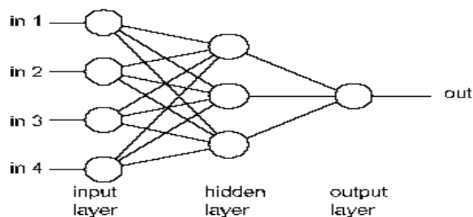
Fig 4: ANN Network
