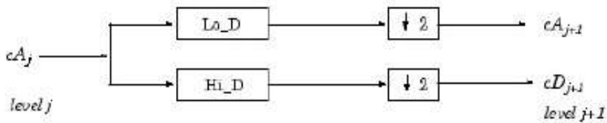
Fig 2 : DWT Framework
