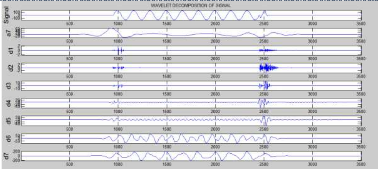
AB fault 0 degree all locations
