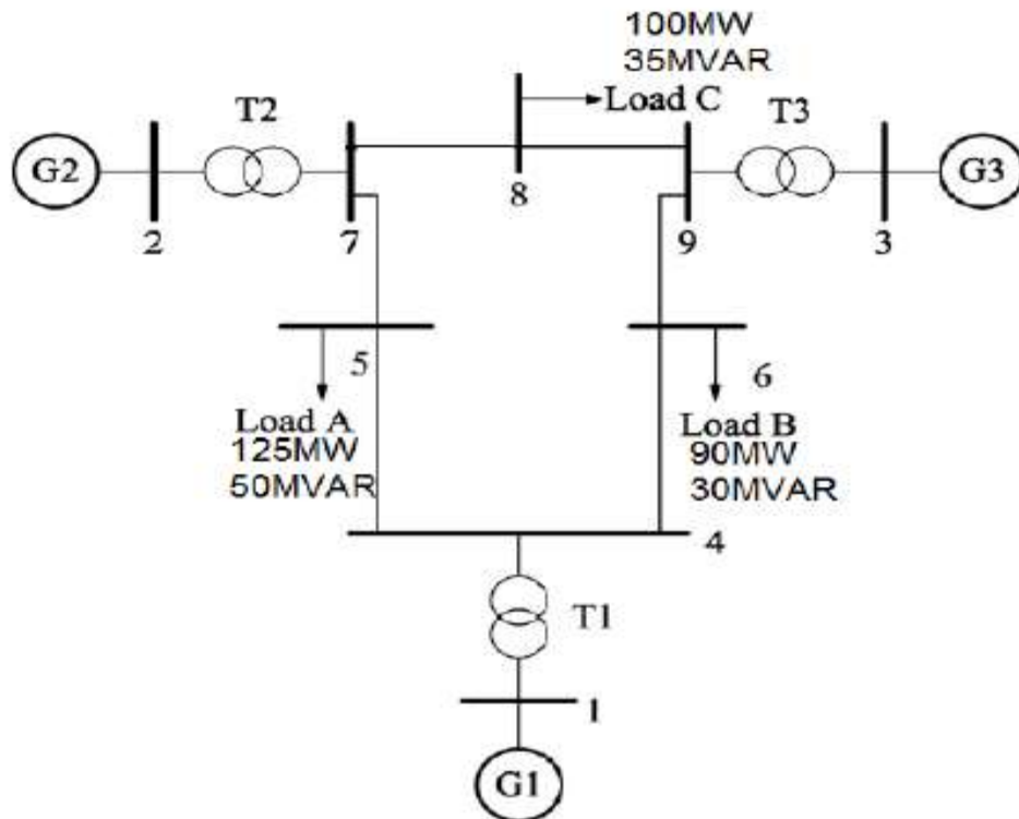
Fig 3 : IEEE 9 Bus System
