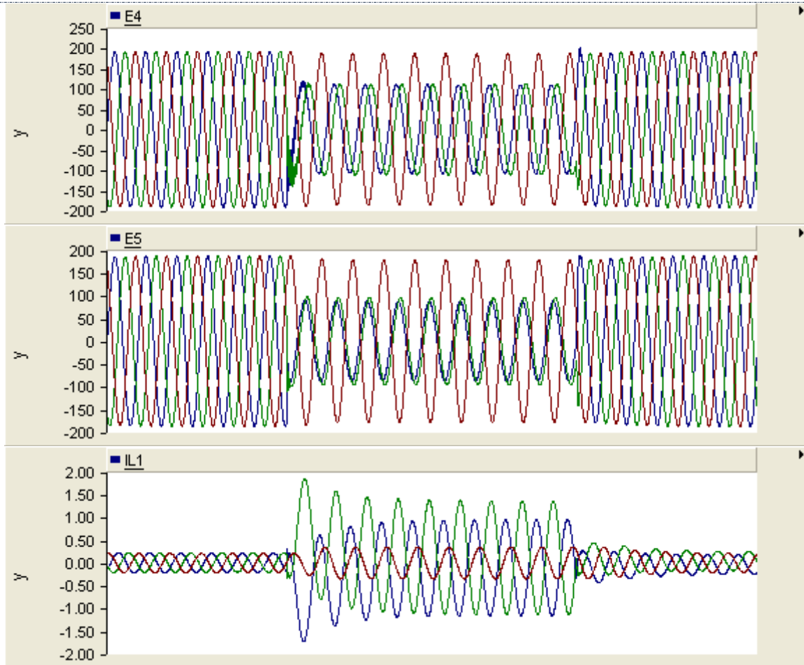
Fig shows the simulation waveforms of line to line fault (L-L) at 0.5 m between bus 4 and bus 5 at an inception angle of 90 degree. The graph shows the nature of voltages of bus 4 i.e E4 and Bus 5 i.e E5 and fault current IL1. The faulted waves of current and voltages can be observed during line to fault.
