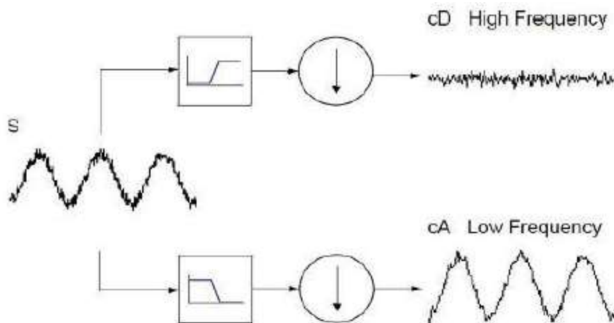
Fig1: Analysis Of Signal using Discrete wavelet Transform
