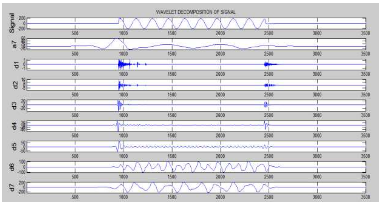
ABG fault 0 degree all locations
