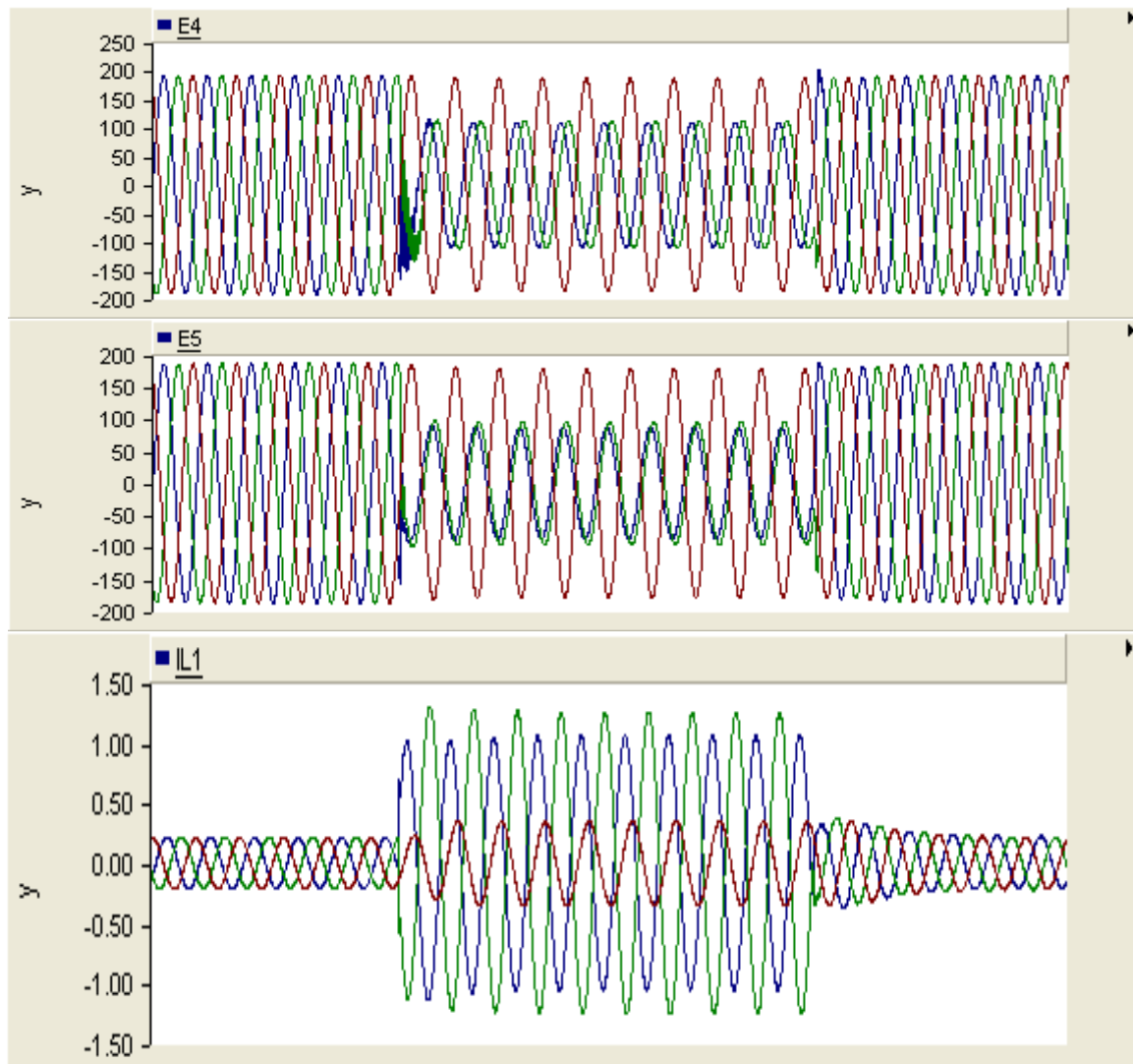
Fig shows the simulation waveforms of line to line fault (L-L) at 0.5 m between bus 4 and bus 5 at an inception angle of 45 degree. The graph shows the nature of voltages of bus 4 i.e E4 and Bus 5 i.e E5 and fault current IL1. The faulted waves of current and voltages can be observed during line to fault.
